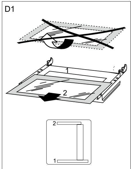
Removal of the internal glass panel 2 glass.
