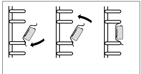
Installing telescopic runners
