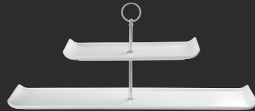
LARGE RECTANGULAR PLATE TOWER* APRBAPT21 Top Plate: 30 x 14.5cm 11 3/4" x 5 1/2" Bottom Plate: 56 x 15.3cm 22" x 6" Height: 22cm 8 1/2" CTN QTY 2
