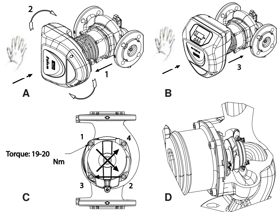
Figure 2: Instructions for motor head assembly
