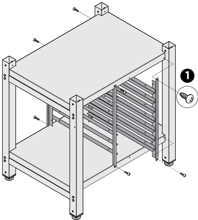
Stand XWVRC-0021-H
