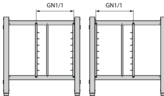
Stand XWVRC-0011-H
